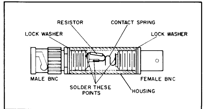
Figure 3. Load Resistor, Cutaway View
